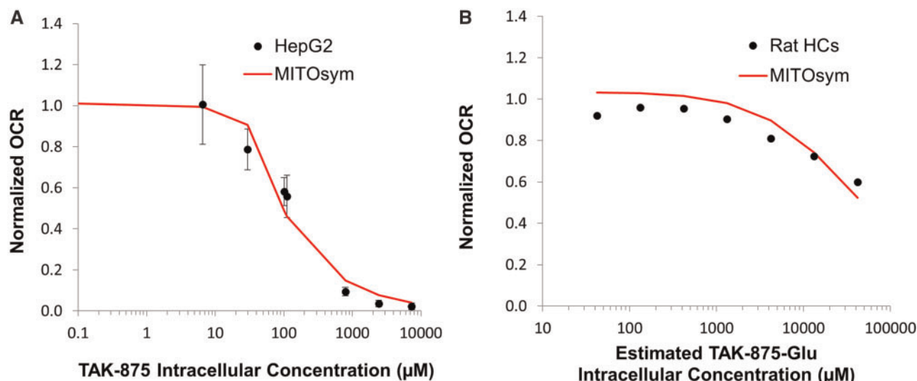
Figure 4. Observed and simulated oxygen consumption rate (OCR) in response to TAK-875 and TAK-875-Glu. A, In vitro respiration data for TAK-875 plotted against intracellular concentrations obtained from HepG2 cells. B, In vitro respiration data for TAK-875-Glu obtained from rat hepatocytes plotted against estimated intracellular concentrations based on simulations using the physiologically based pharmacokinetic (PBPK) sub-model for TAK-875. The results of simulated OCR responses for TAK-875 and TAK-875-Glu conducted in MITOSym are overlaid on both graphs.
