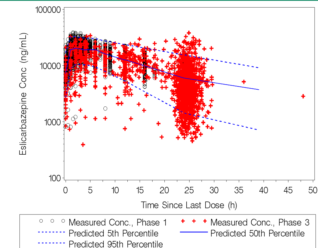
Figure 4. Percentiles of Simulated Data From the Visual Predictive Check of the Final Model Overlaid on the Observed Eslicarbazepine Concentration Data
