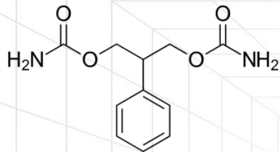
Felbamate: Anti-convulsant
