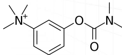
Noestigmine: Neuro-degenerative
