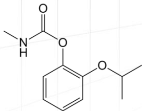
Propoxur: Insecticide
