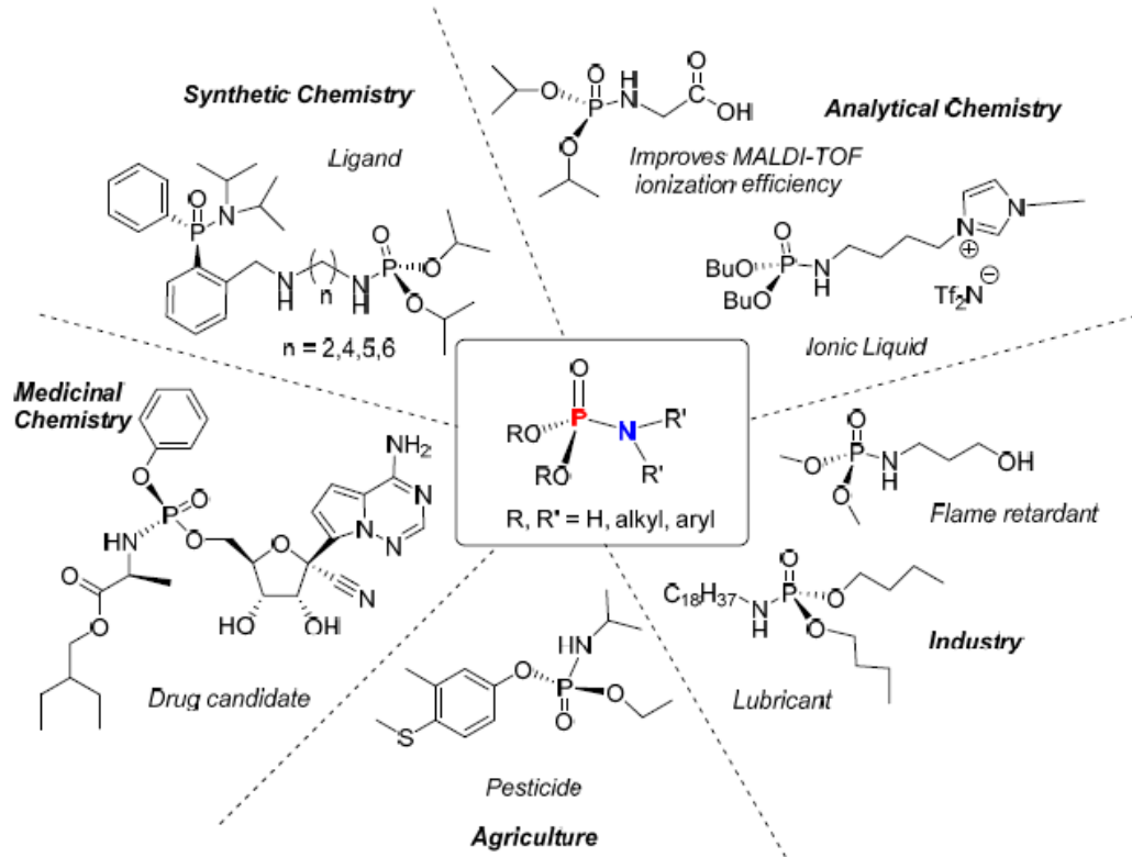
Figure 3. Applications of phosphoramidates.
